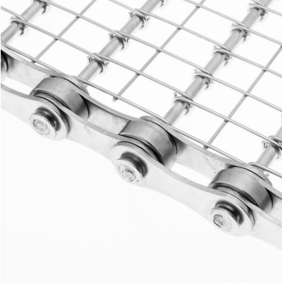
EYE LINK WITH ELECTRO WELDED ROD CONVEYOR BELT AND CHAIN (CMG-VE)
